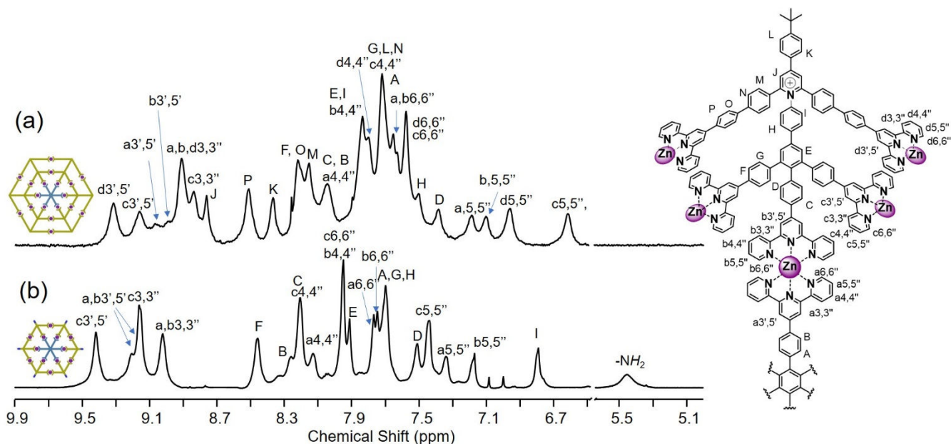
Figure 4. 1 H NMR spectra (600 MHz, d 6 -DMSO, 300 K) of (a) SW-1 and (b) SW-3 .
