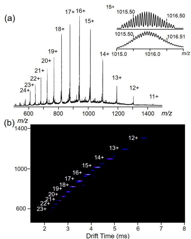
Figure 1. (a) Full ESI-MS spectrum with theoretical and experimental isotope patterns of 15+ species (right inset). (b) TWIM-MS ( m/z vs drift time) of KC composed by three-component in-situ self-assembly strategy.
